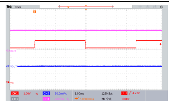
Line Transient@3.3V, IOUT=500mA
