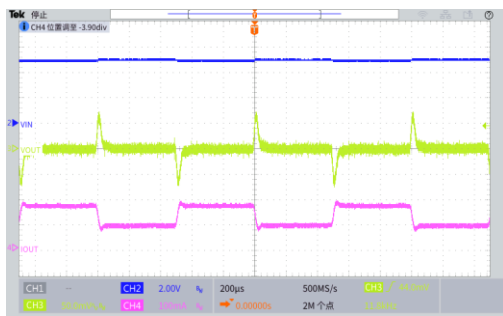
图 1 Load Transient (VIN=5V, IOUT=75mA-150mA-75mA)
