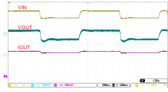
图 2 Line Transient ( V_{IN} =from V_{OUT}+1V to 7V to V_{OUT}+1V , I_{OUT}=1A )
