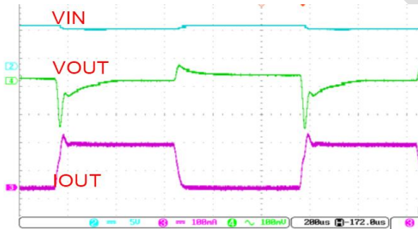
图 3 Load Transient (VIN=7V, IOUT=0mA-150mA-0mA)
