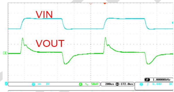
图 2 Line Transient (VIN=from 5.6V to 7V to 5.6V IOUT=150mA)
