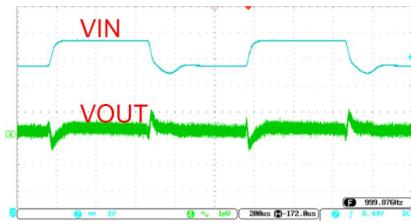
图 1 Line Transient (VIN=from 5.6V to 12V to 5.6V IOUT=0mA)
