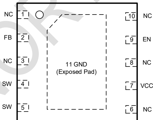
DFN3 \times 3-10L
