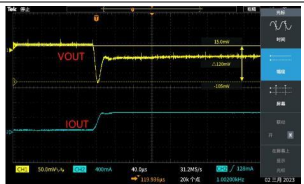
图 6 Load Transient ( V_{IN}=V_{OUT}+1V , I_{OUT}=500mA-50mA )
